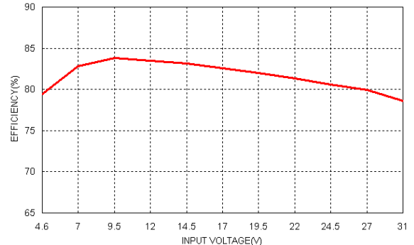
SSR01-12S05 -5Vout EFFICIENCY VS INPUT VOLTAGE
