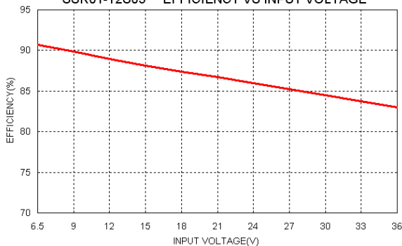
SSR01-12S05 EFFICIENCY VS INPUT VOLTAGE
