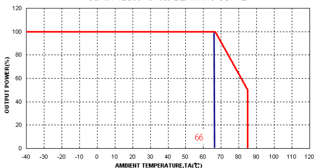
SSR01-12S05 -5Vout DERATING CURVE
