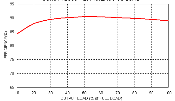
SSR01-12S05 EFFICIENCY VS LOAD
