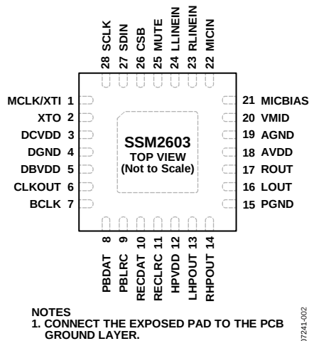
Figure 6. Pin Configuration
