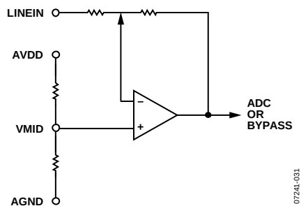
Figure 19. Line Input to ADC
