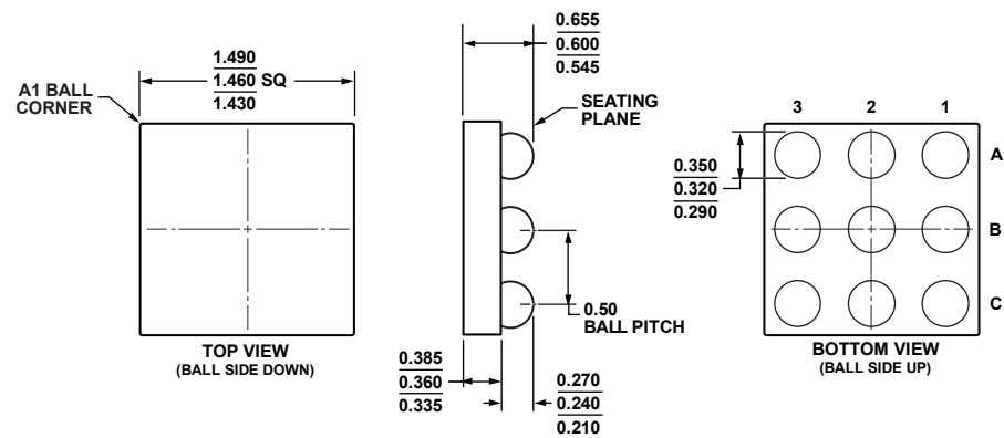
Figure 42. 9-Ball Wafer Level Chip Scale Package [WLCSP] (CB-9-2) Dimensions shown in millimeters
