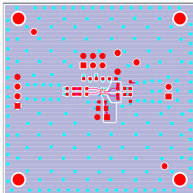
Figure 6. Top Layer
