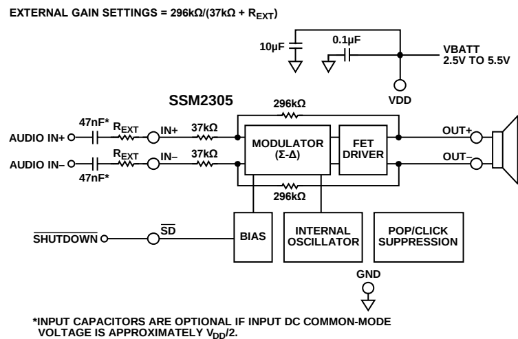
Figure 32. Differential Input Configuration, User-Adjustable Gain
