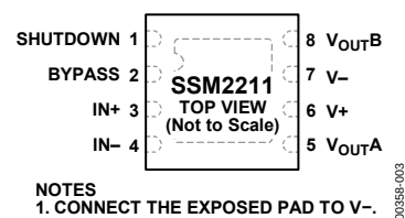
Figure 3. 8-Lead LFCSP Pin Configuration (CP-8-13)
