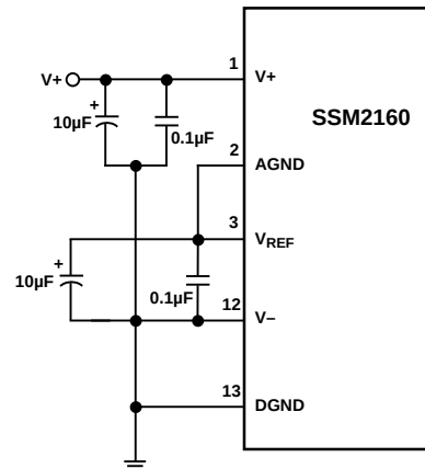
Figure 15. Single Supply Configuration
