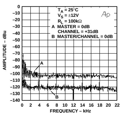
Figure 11. Noise Floor FFT
