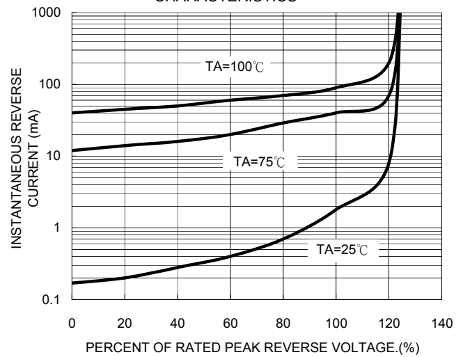
FIG. 4 TYPICAL RERVERSE CHARACTERISTICS
