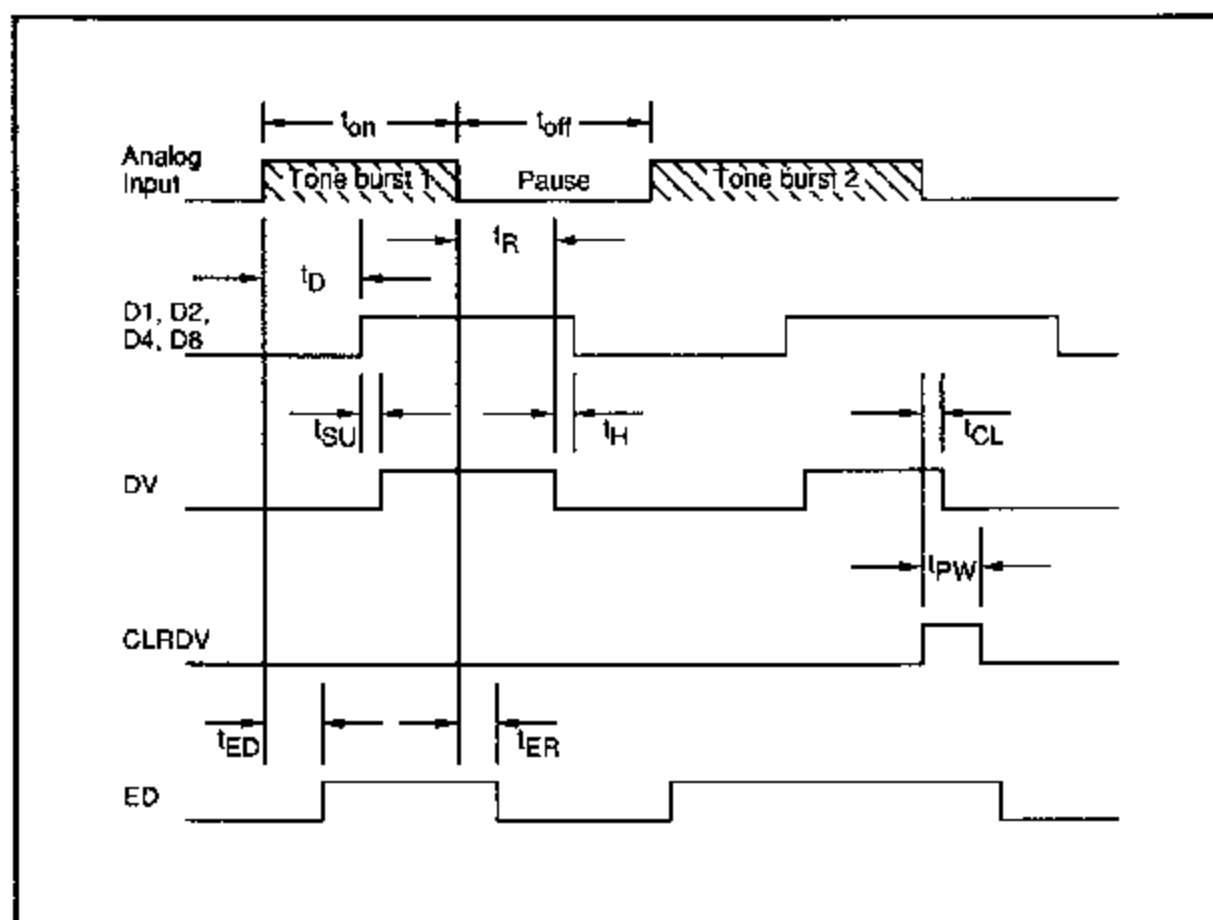
FIGURE 4: Timing Diagram
