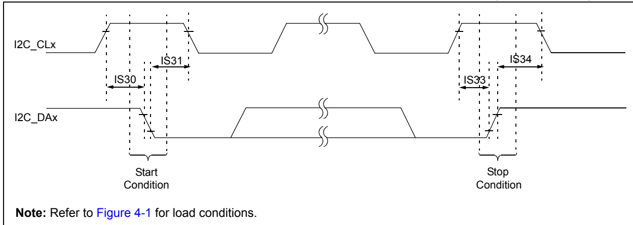
FIGURE 4-6: I 2 Cx BUS START/STOP BITS TIMING CHARACTERISTICS (SLAVE MODE)
