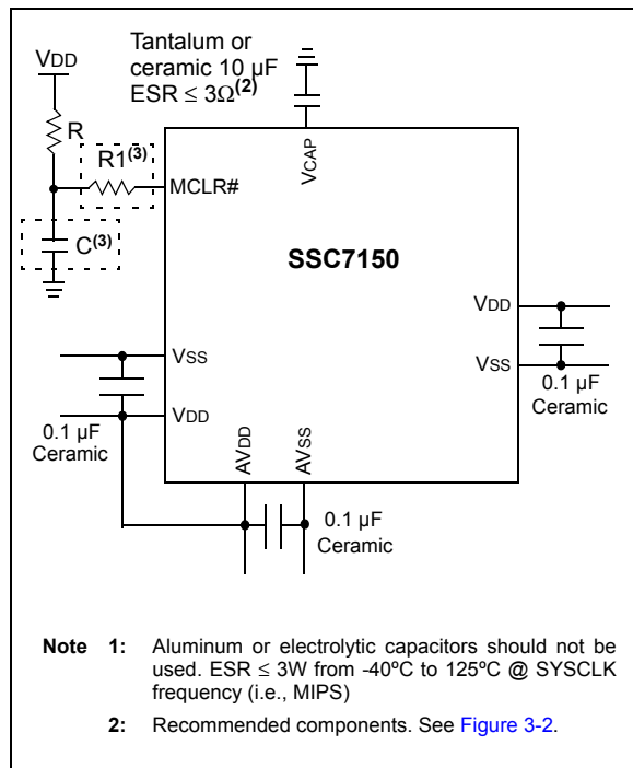
FIGURE 3-1: RECOMMENDED MINIMUM CONNECTION
