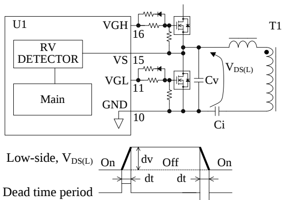
Figure 8-26. VS pin and dead time period
