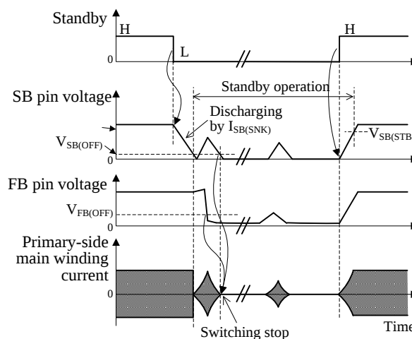
Figure 8-21. Standby change operation waveforms
