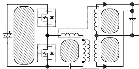
Figure 9-3. High frequency current loops (hatched areas)
