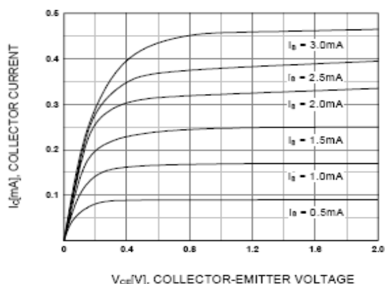
Figure 1. Static Characteristic
