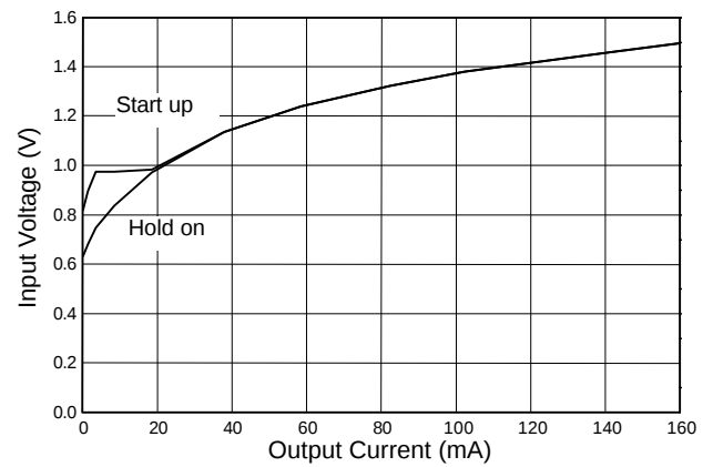
Fig. 12 SS6639-50 Start-up & Hold-on Voltage (L=33uH)
