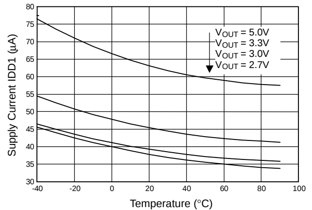
Fig. 18 SS6639 Supply Current vs. Temperature
