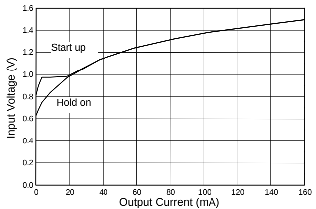
Fig. 14 S6639-50 Start-up & Hold-on Voltage (L=33uH)
