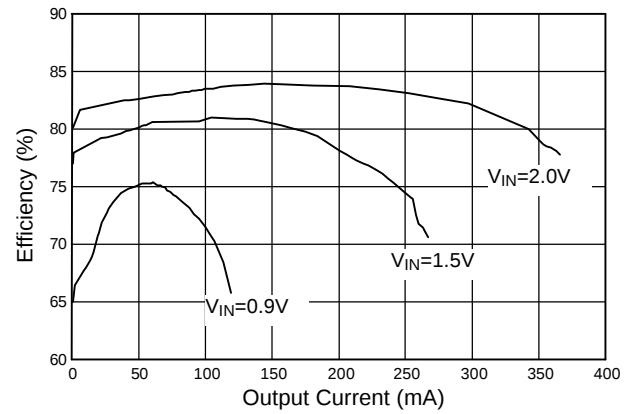
Fig. 6 SS6639-33 Efficiency (L=33 H)
