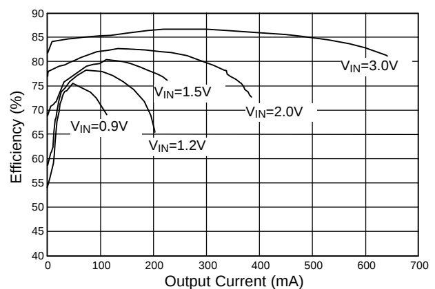
Fig. 8 SS6639-50 Efficiency (L=33 H)
