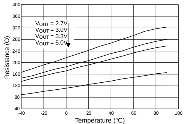
Fig. 20 SS6639 EXT "H" On-Resistance
