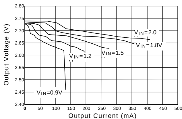
Fig. 1 SS6639-27 Load Regulation (L=33 H)
