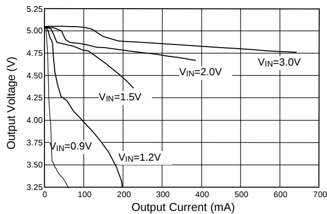
Fig. 7 SS6639-50 Load Regulation (L=33μH)
