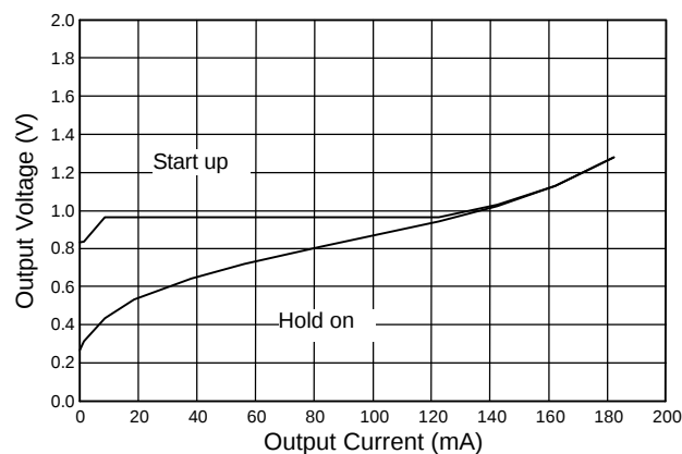
Fig. 9 SS6639-27 Start-up & Hold-on Voltage (L=33μH)
