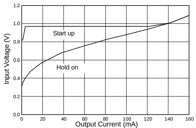
Fig. 10 SS6639-30 Start-up & Hold-on Voltage (L=33 H)
