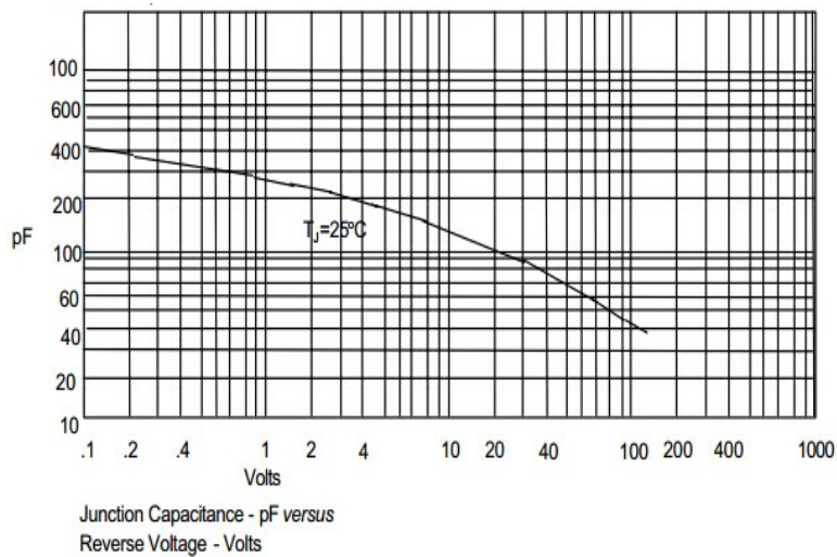
FIG.4-TYPICAL JUNCTION CAPACITANCE
