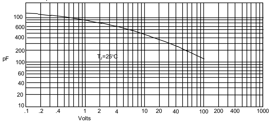
Figure 3 Junction Capacitance
