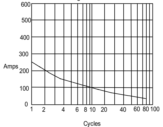
Figure 5 Peak Forward Surge Current
