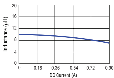
SRN3010TA-100M
