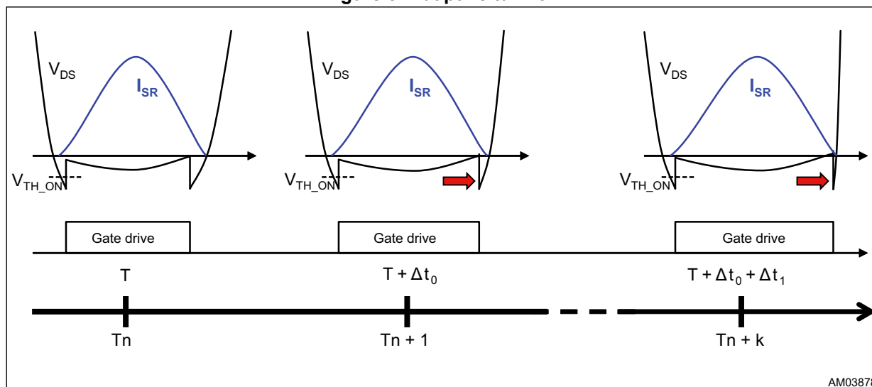
Figure 8. Adaptive turn-off
