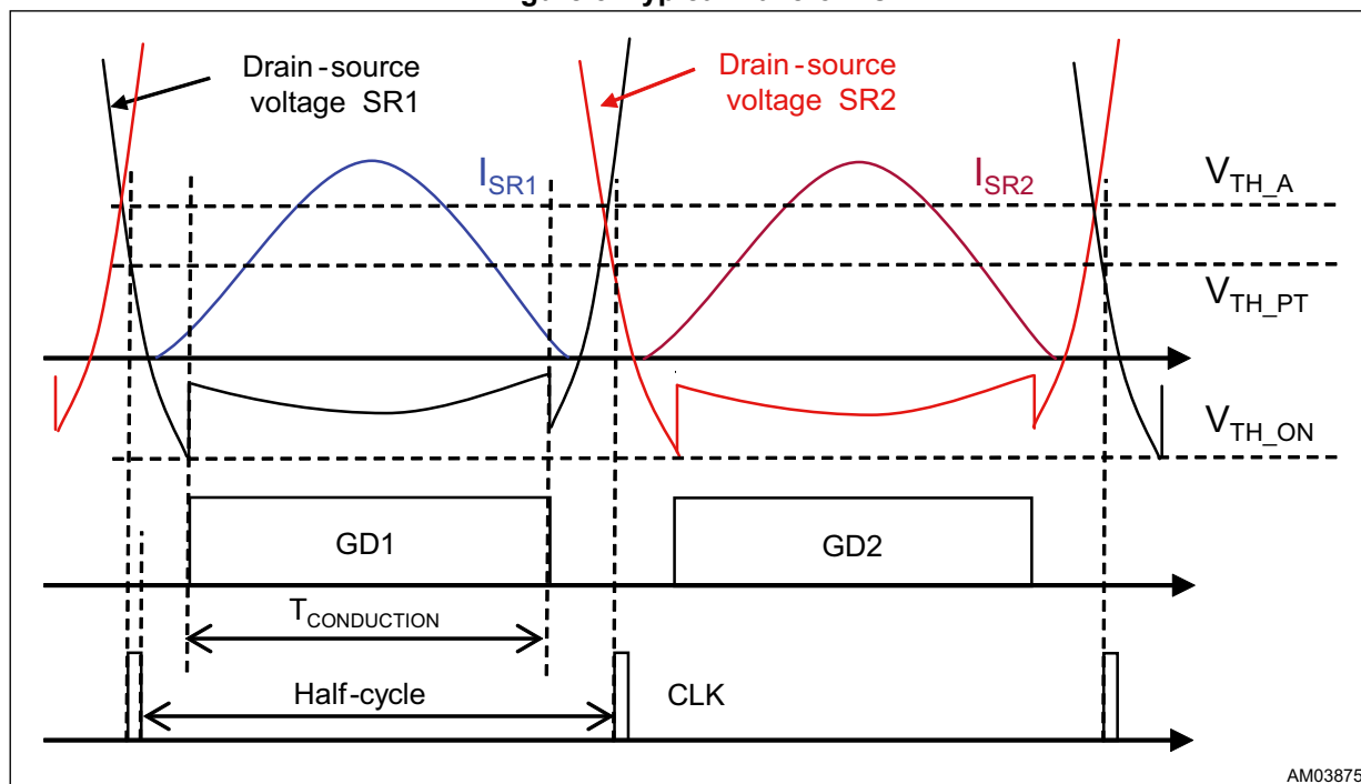
Figure 5. Typical waveforms
