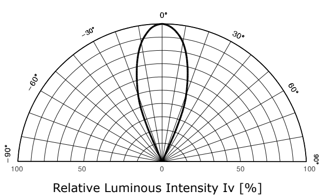
Fig. 5 Radiation Diagram
