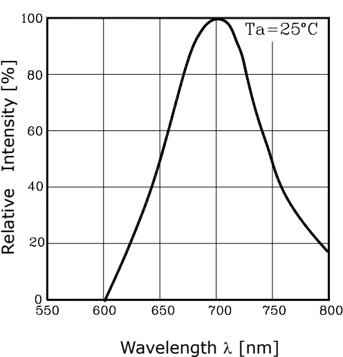
Fig. 4 Spectrum Distribution
