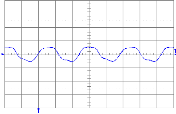
Fig. 6.0V.13: Output voltage ripple (50 mV/div.) at full rated load current into a resistive load with C_o = 10 \mu\text{F} tantalum + 1\mu\text{F} ceramic and V_{in} = 24 \text{ V} . Time scale: 1 \mu\text{s}/\text{div} .
