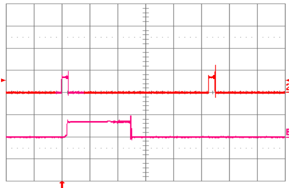
Fig. 6.0V.18: Load current (top trace, 20 \text{ A}/\text{div.} , 20 \text{ ms}/\text{div.} ) into a 10 \text{ m}\Omega short circuit during restart, at V_{in} = 24 \text{ V} . Bottom trace ( 20 \text{ A}/\text{div.} , 2 \text{ ms}/\text{div.} ) is an expansion of the on-time portion of the top trace.
