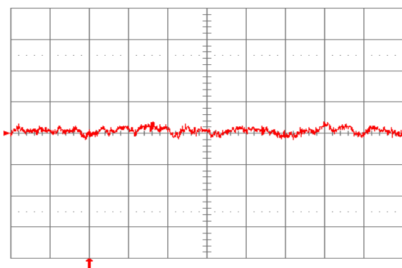
Fig. 1.0V.16: Input reflected ripple current, i_s (10 mA/div.), measured through 10 \mu\text{H} at the source at full rated load current and V_{in} = 24 \text{ V} . Refer to Fig. 1.0V.14 for test setup. Time scale: 1 \mu\text{s}/\text{div} .
