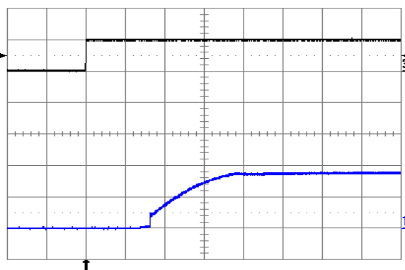
Fig. 1.8V.10: Turn-on transient at full rated load current (resistive) plus 10,000 \mu\text{F} at V_{in} = 24\text{V} , triggered via ON/OFF pin. Top trace: ON/OFF signal (5 V/div.). Bottom trace: output voltage (1 V/div.). Time scale: 1 ms/div.
