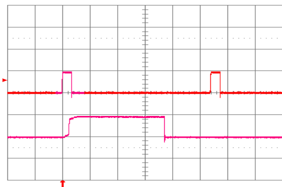
Fig. 1.0V.18: Load current (top trace, 20 \text{ A}/\text{div} ., 20 \text{ ms}/\text{div} .) into a 10 \text{ m}\Omega short circuit during restart, at V_{in} = 24 \text{ V} . Bottom trace ( 20 \text{ A}/\text{div} ., 2 \text{ ms}/\text{div} .) is an expansion of the on-time portion of the top trace.
