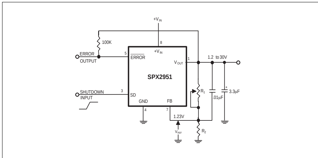
Figure 2. Adjustable Regulator
