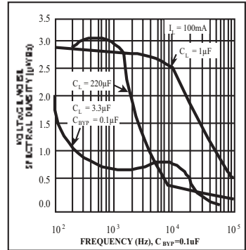
Output Noise
