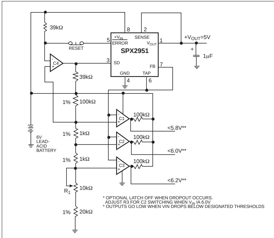
Figure 6. Regulator with State-of-Charge Indicator
