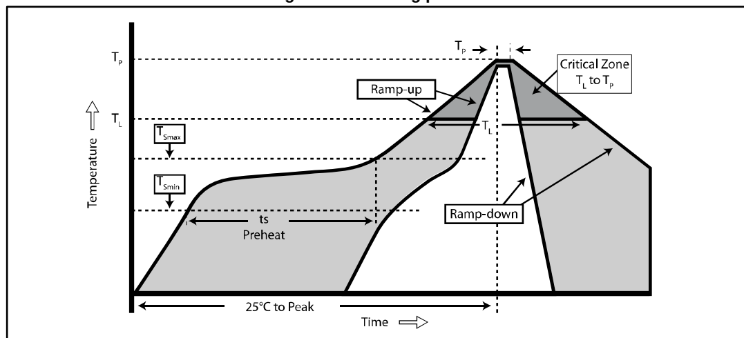
Figure 6: Soldering profiles
