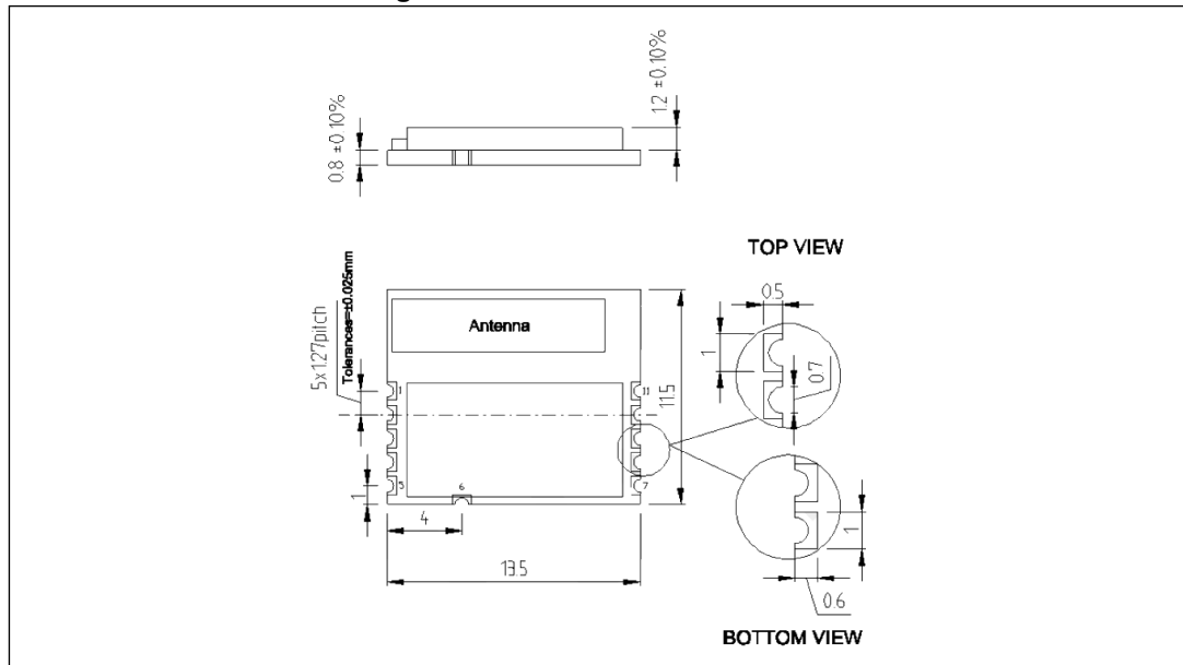
Figure 4. Mechanical dimensions
