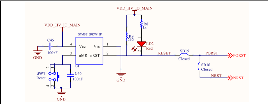
Figure 11. Reset circuit
