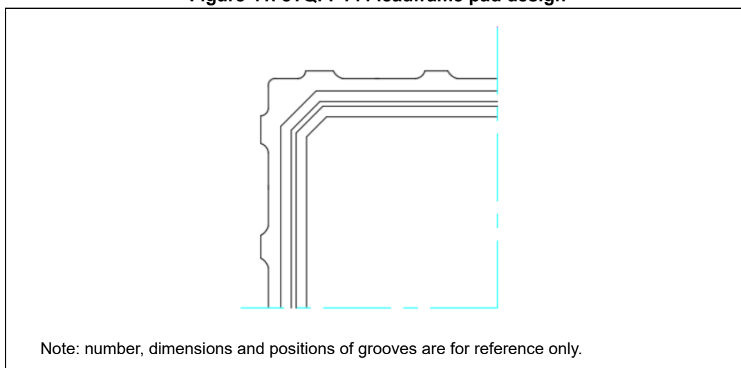
Figure 41. eTQFP144 leadframe pad design
