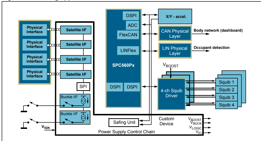
Figure 3. Airbag application
