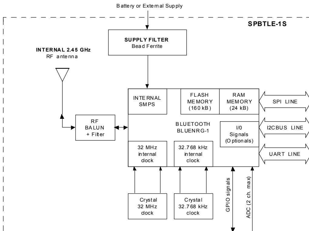
Figure 1. Block diagram
