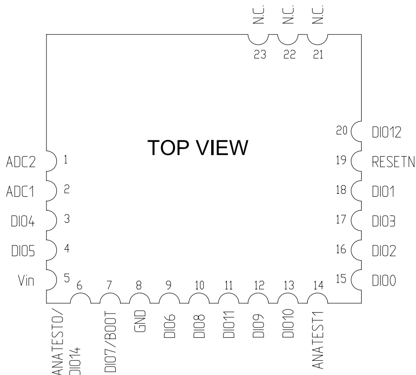
Figure 7. Pin assignment
