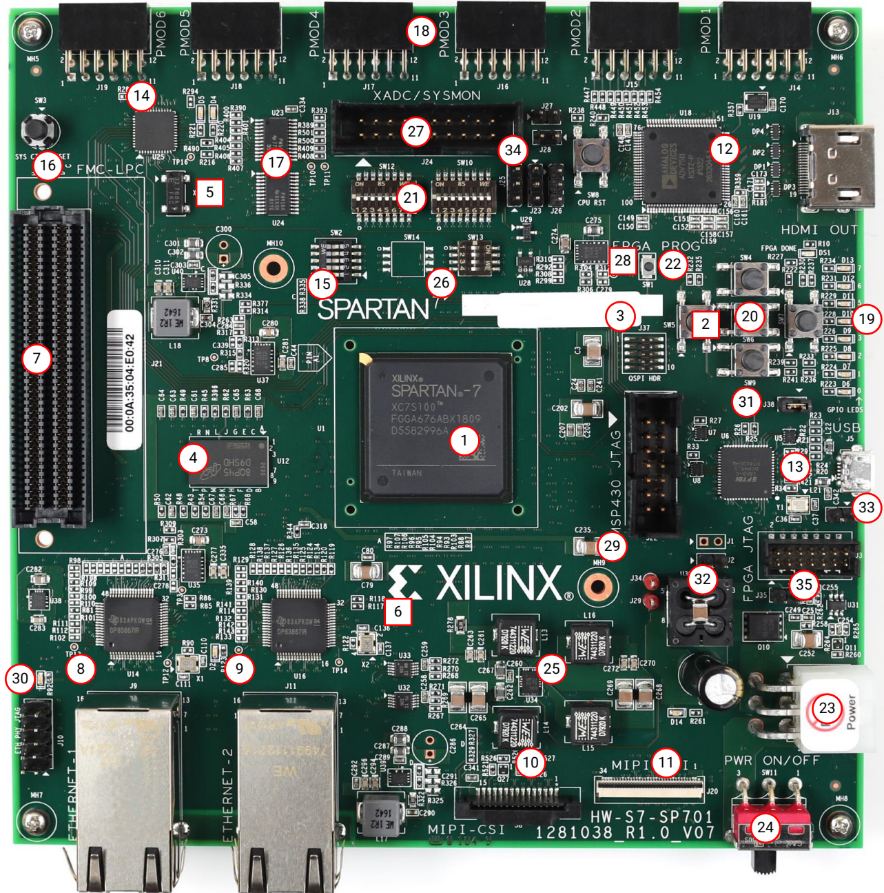
○ Round callout references a component on the front side of the board ◻ Square callout references a component on the back side of the board
