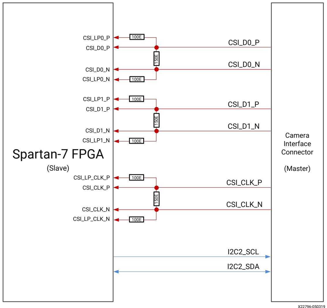
Figure 14: MIPI-CSI Interface
