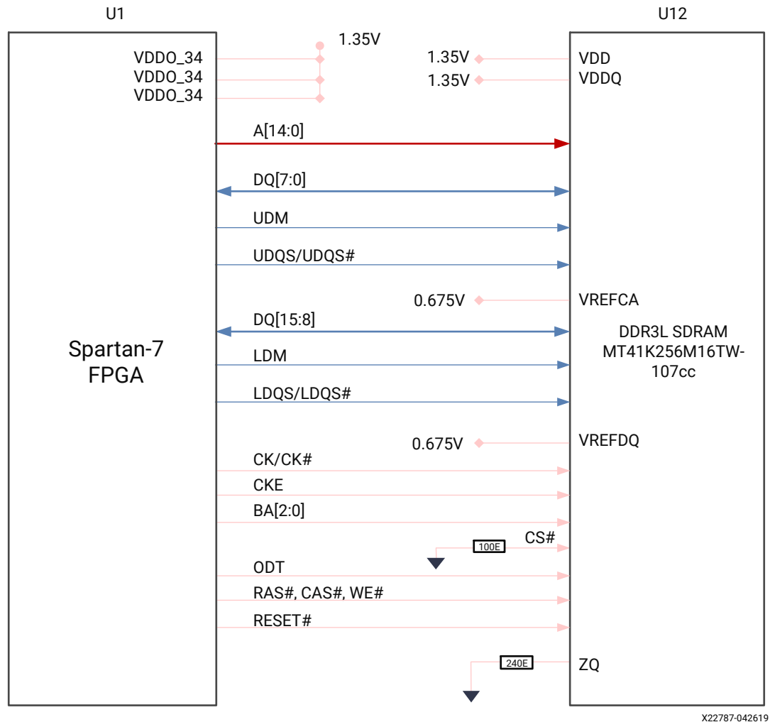
Figure 4: DDR3L Memory Interface
