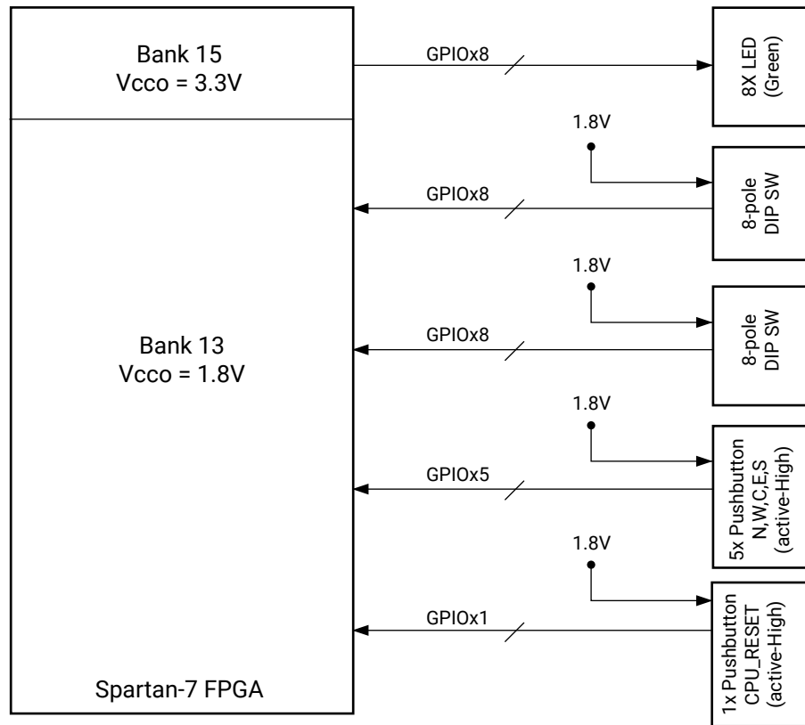
Figure 16: User GPIO
