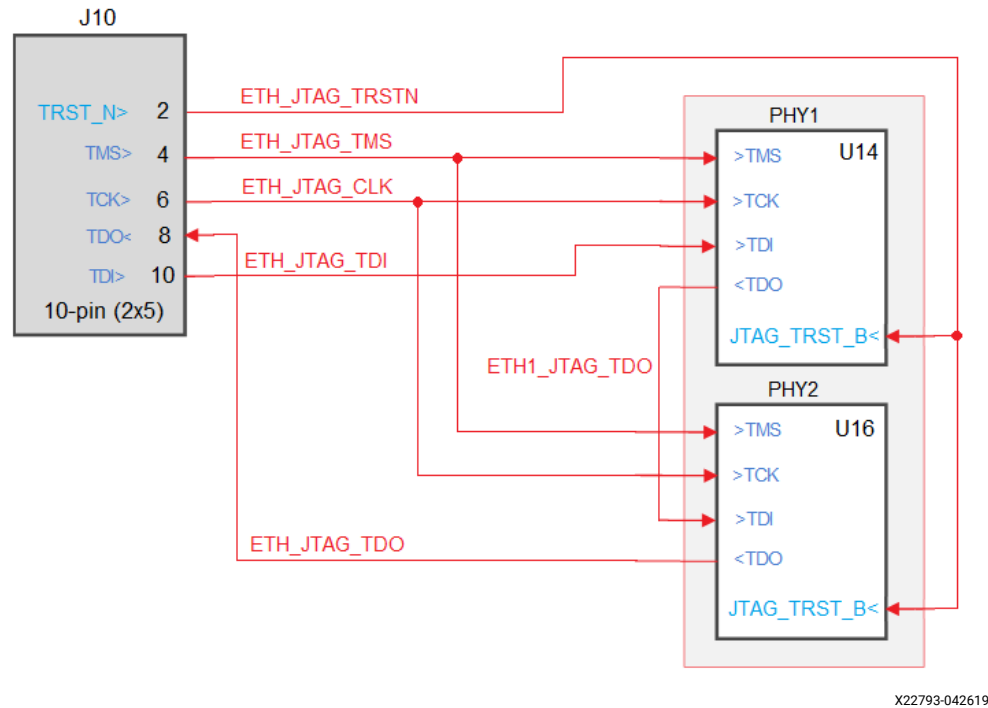
Figure 10: Ethernet JTAG
