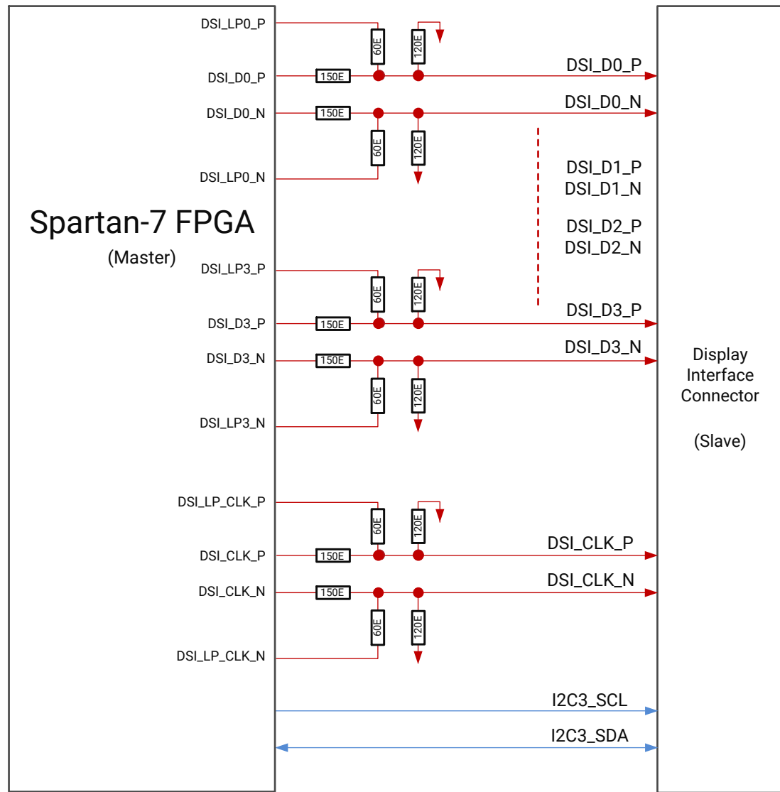
Figure 15: MIPI-DSI Interface
