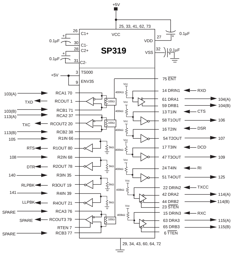
Figure 27. Typical DCE V.35 Interface
