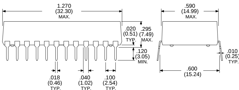
Default Thru-hole 24-Pin Package. Example: SP24A-105
