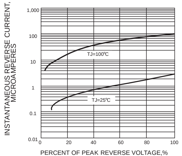
FIG. 4-TYPICAL REVERSE CHARACTERISTICS
