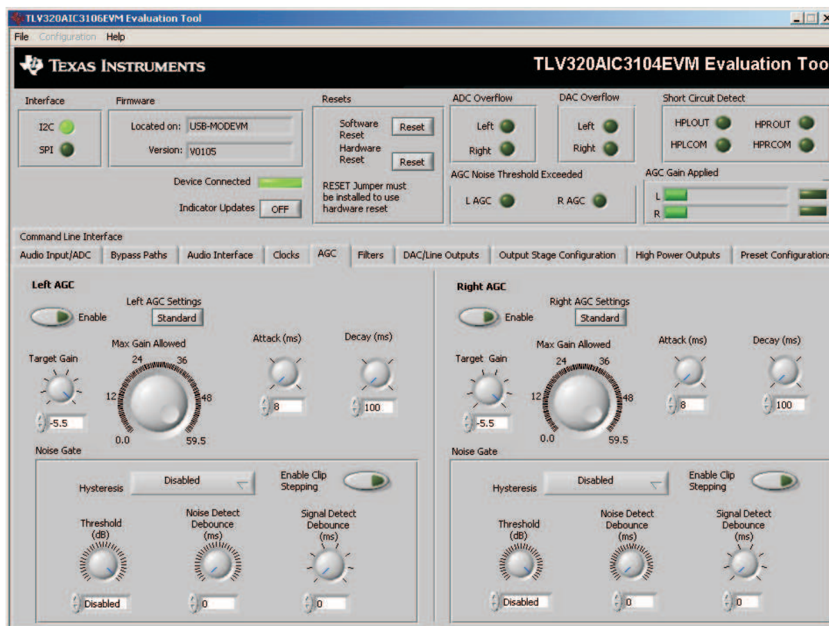
Figure 12. AGC Tab
