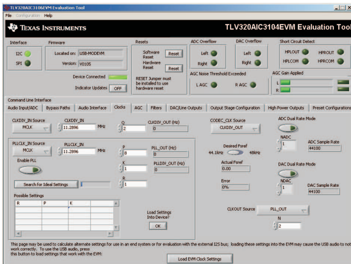
Figure 10. Clocks Tab
