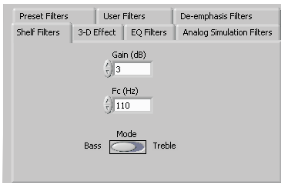
Figure 21. Shelf Filters
