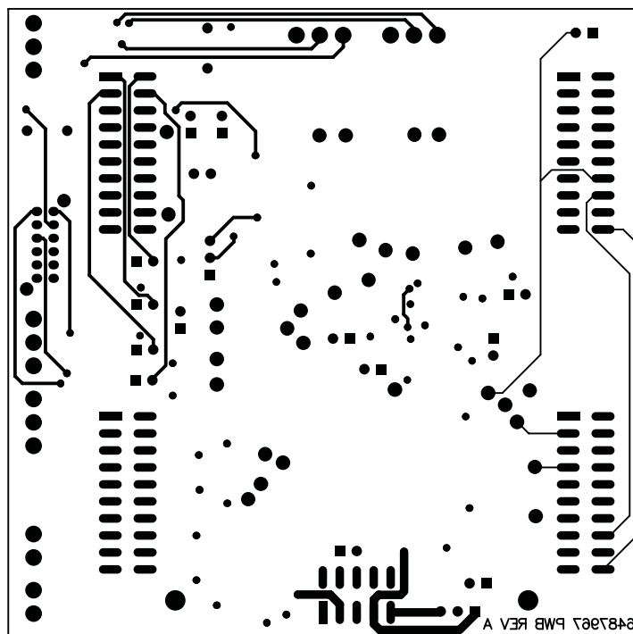
Figure C-5. Silk Screen
