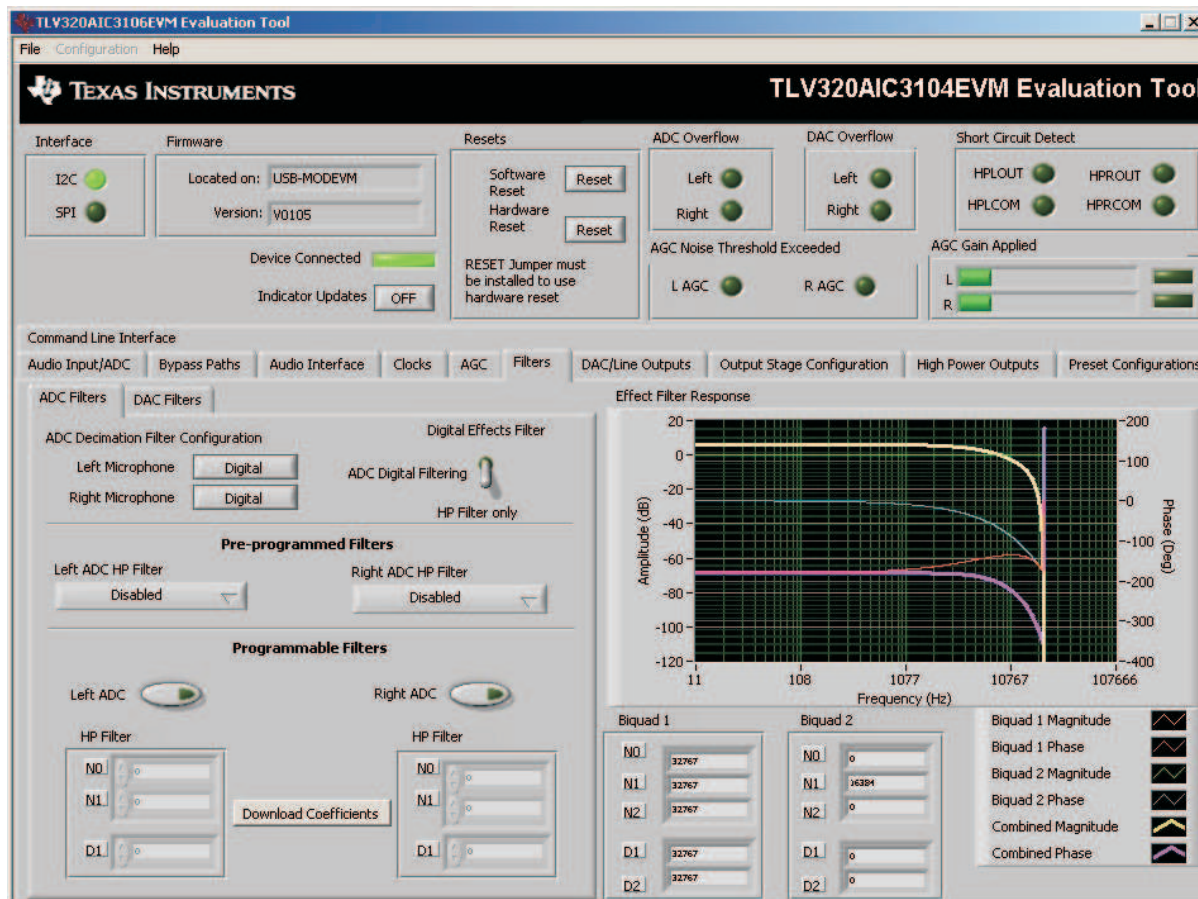
Figure 15. Filters Tab
