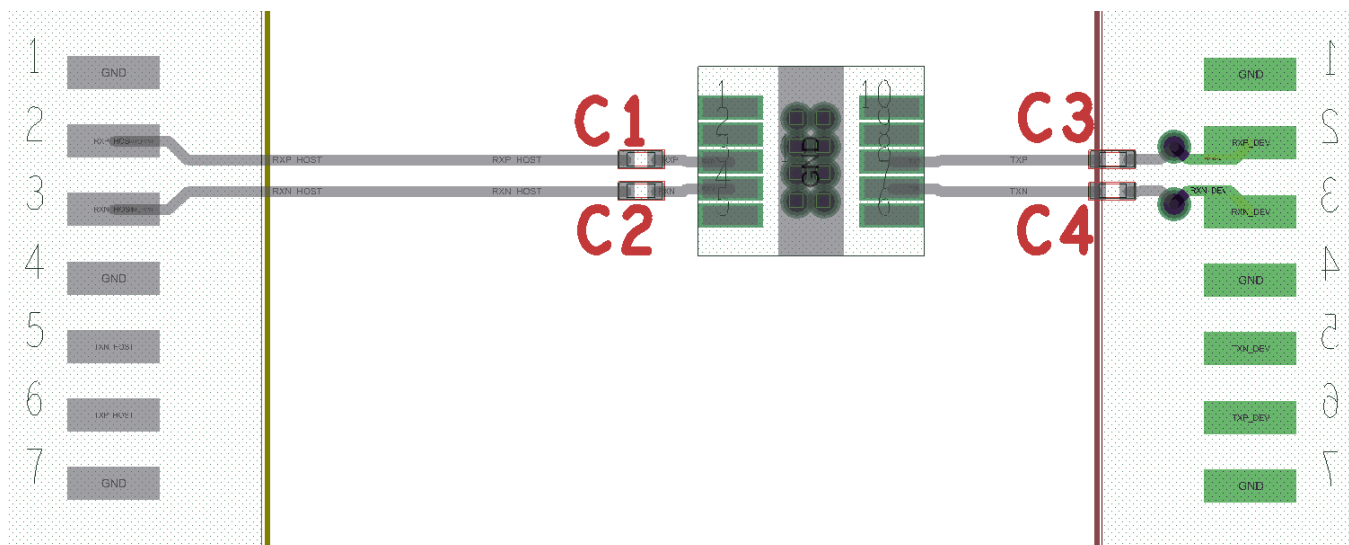
Figure 30. Example Layout
