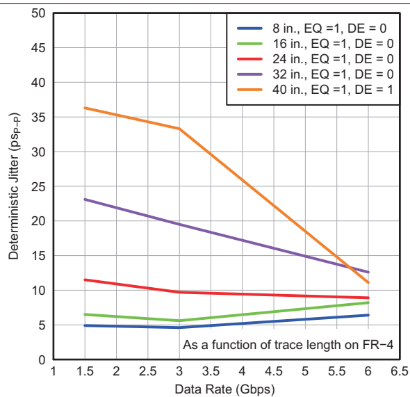
Figure 8. SAS-Mode Deterministic Jitter vs Data Rate
