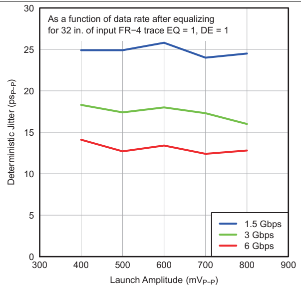
Figure 7. SATA-Mode Deterministic Jitter vs Launch Amplitude
