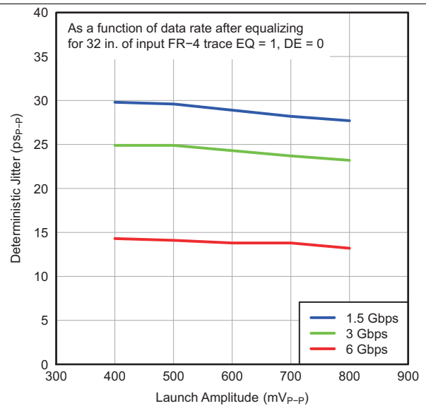
Figure 9. SAS-Mode Deterministic Jitter vs Launch Amplitude
