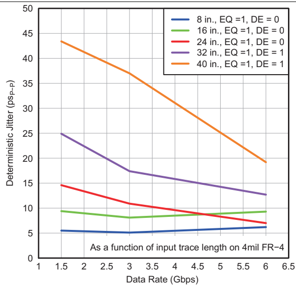
Figure 6. SATA-Mode Deterministic Jitter vs Data Rate
