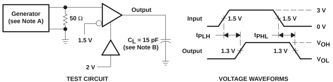
Figure 1. V_{OH} , V_{OL}
