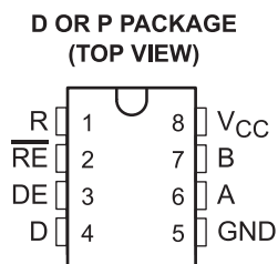
Pin Functions
