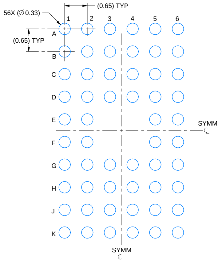
LAND PATTERN EXAMPLE EXPOSED METAL SHOWN SCALE:15X
