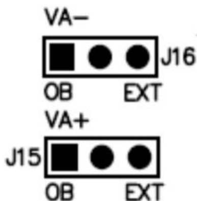
Figure 3. Connectors J15, J16
