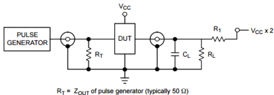
Figure 4. Test Circuit
