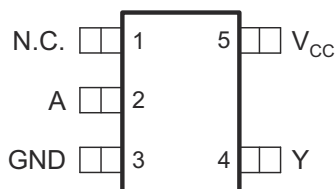
图 5-1. DCK Package 5-Pin SC70 (Top View)
