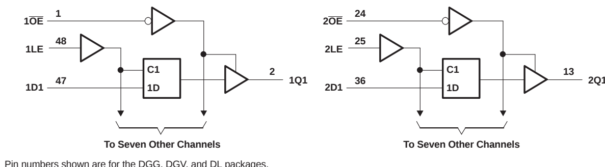
Figure 4. Logic Diagram (Positive Logic)
