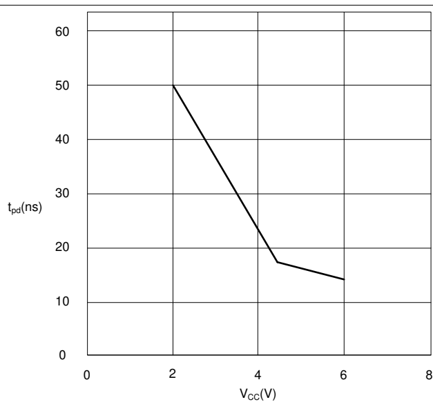
Figure 12. SN75HC595-Q1 t pd vs. V CC
