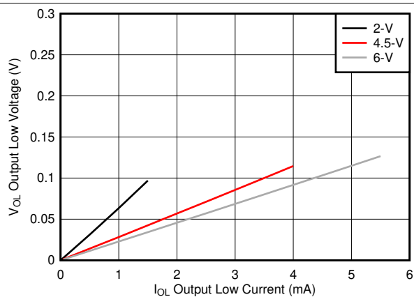
Figure 3. Output voltage versus output current in low state
