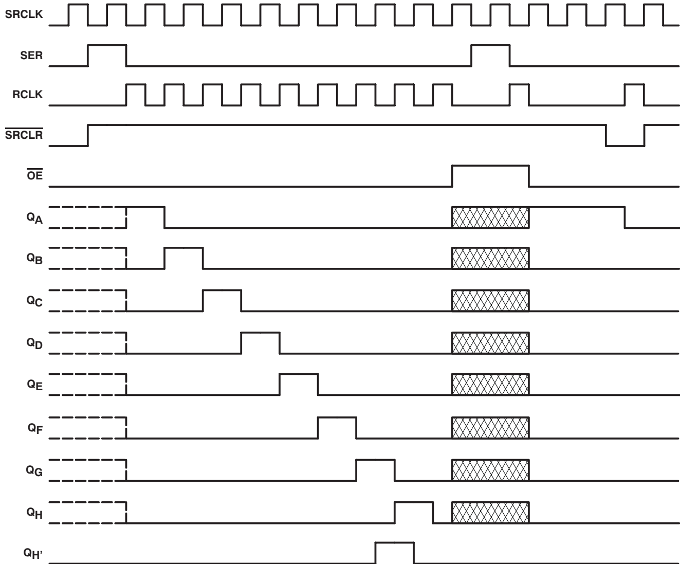
Figure 2. Timing Diagram
