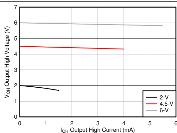
Figure 4. Output voltage versus output current in high state
