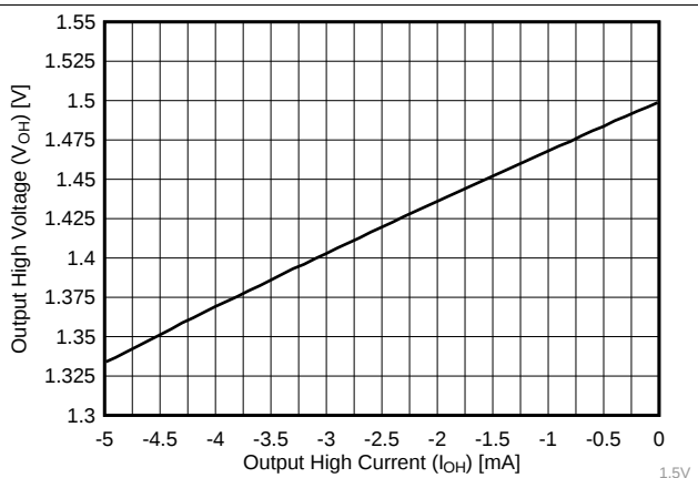
Figure 6. Typical Output High Voltage of 1.5 V (25°C)
