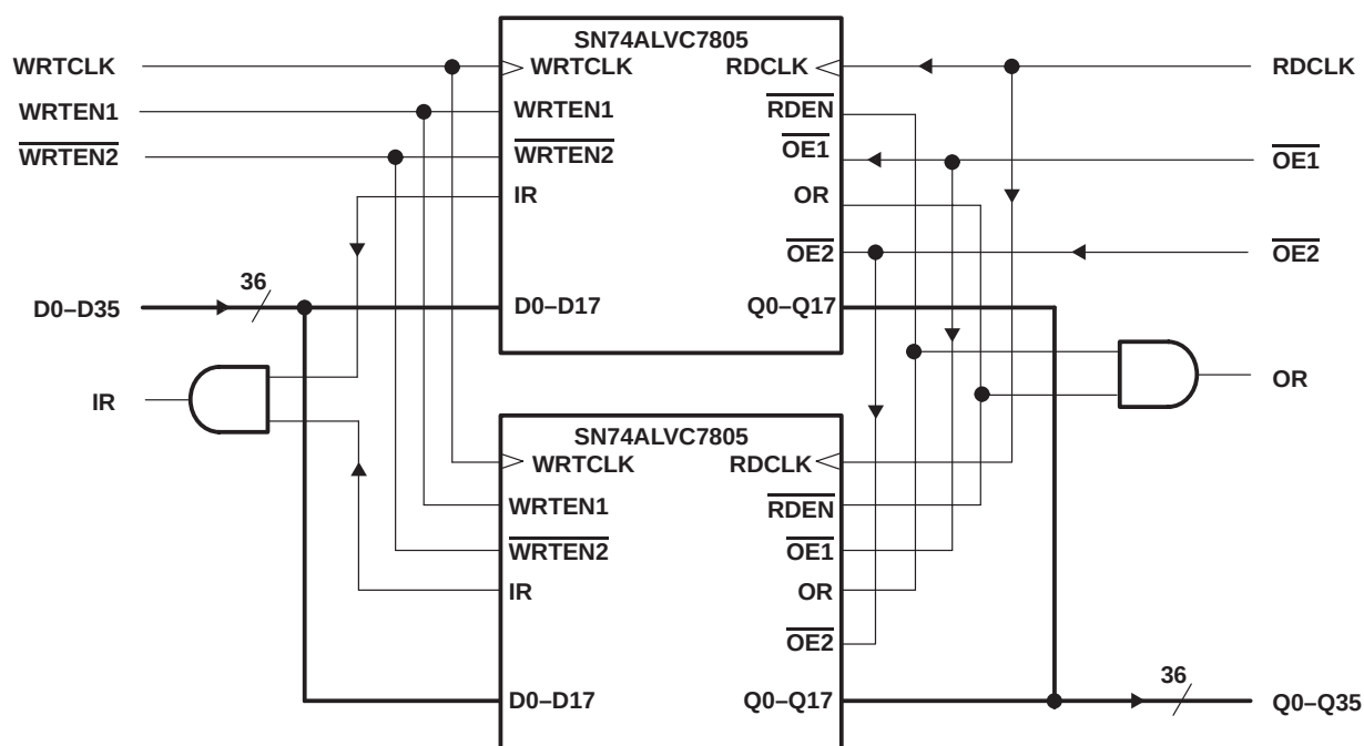
Figure 8. Word-Width Expansion: 256 \times 36 Bits
