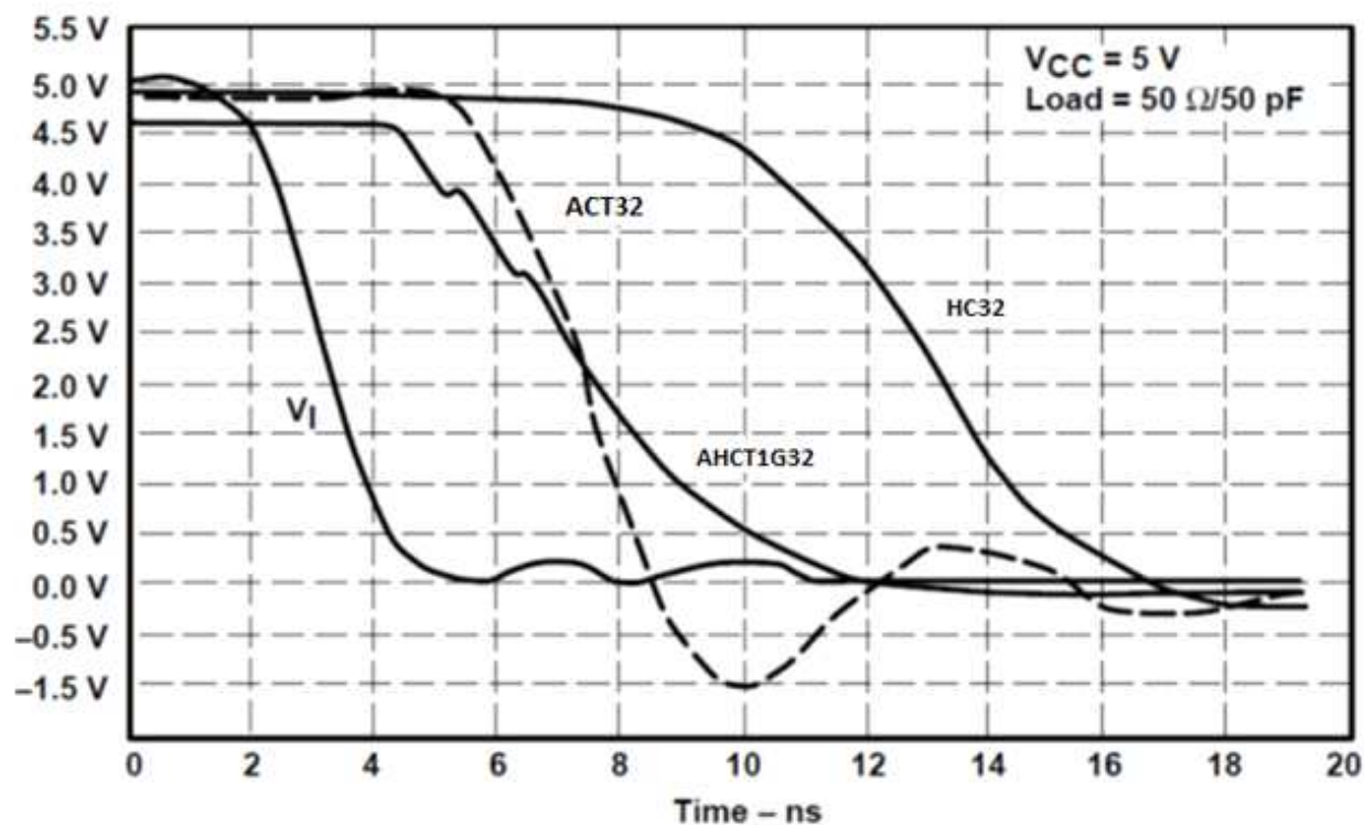
Figure 5. Switching Characteristics Comparison
