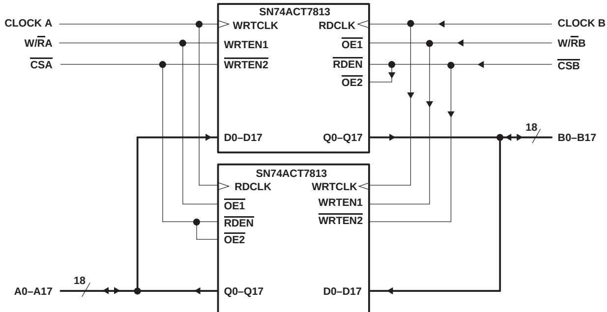
Figure 8. Bidirectional Configuration
