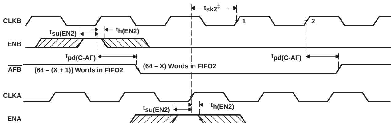
Figure 12. Timing for AFA When FIFO1 Is Almost Full
