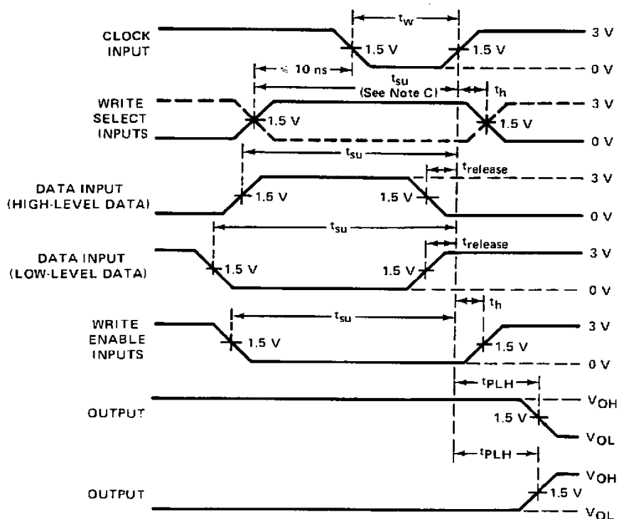
VOLTAGE WAVEFORMS FIGURE 2
