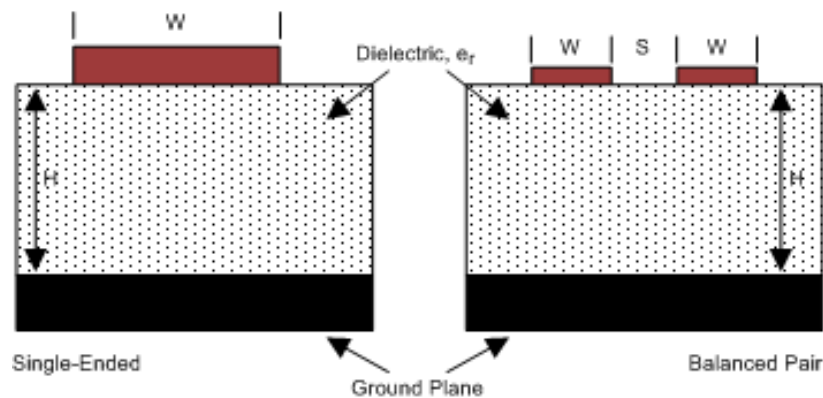
Figure 32. Microstrip Topology
