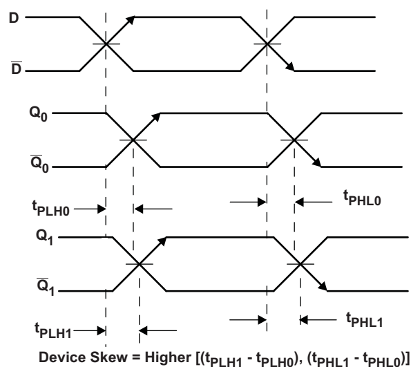
Figure 5. Device Skew
