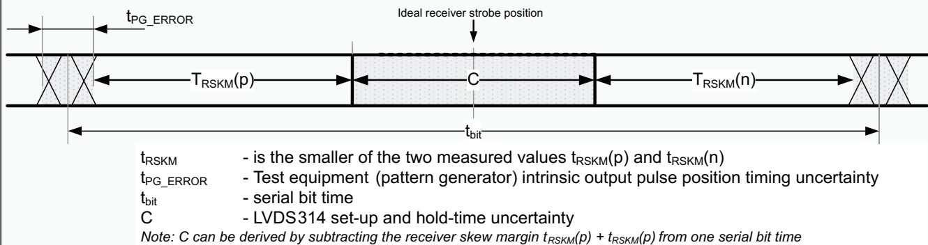
Figure 8. Jitter Budget
