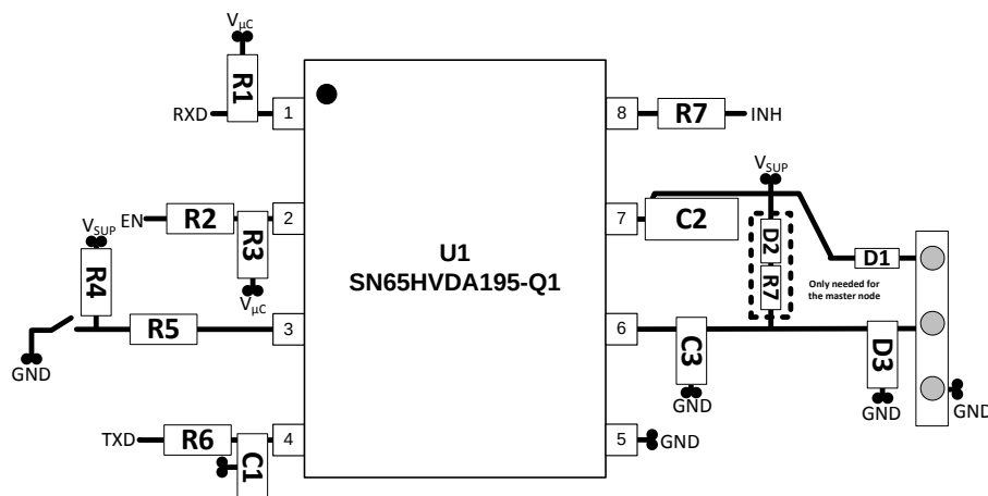
Figure 13. Layout Example
